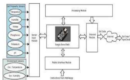
Figure 2: Sensor-Kit Module.
